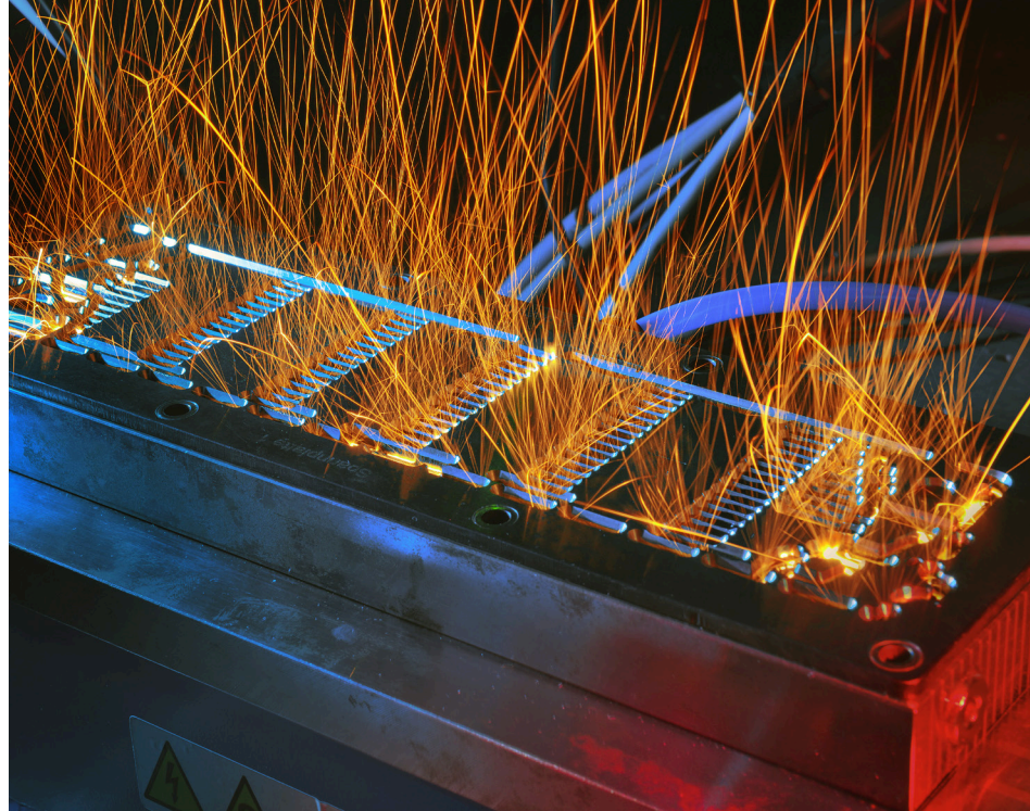
1 Setup with two RAYLASE AS-Fiber 30 scanners. 2 Welding a bipolar plate.
