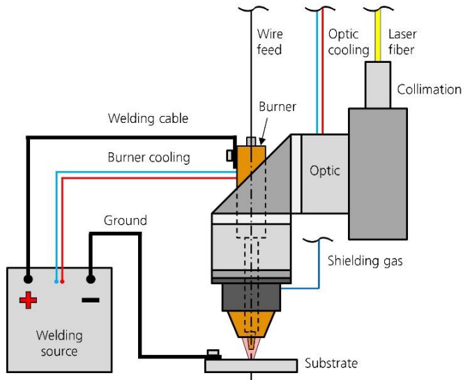
Image 2: Schematic setup of the COLLAR (coaxial laser arc) Hybrid processing head. © Fraunhofer ILT, Aachen, Germany / Max Fabian Steiner and Lukas Rießner.
