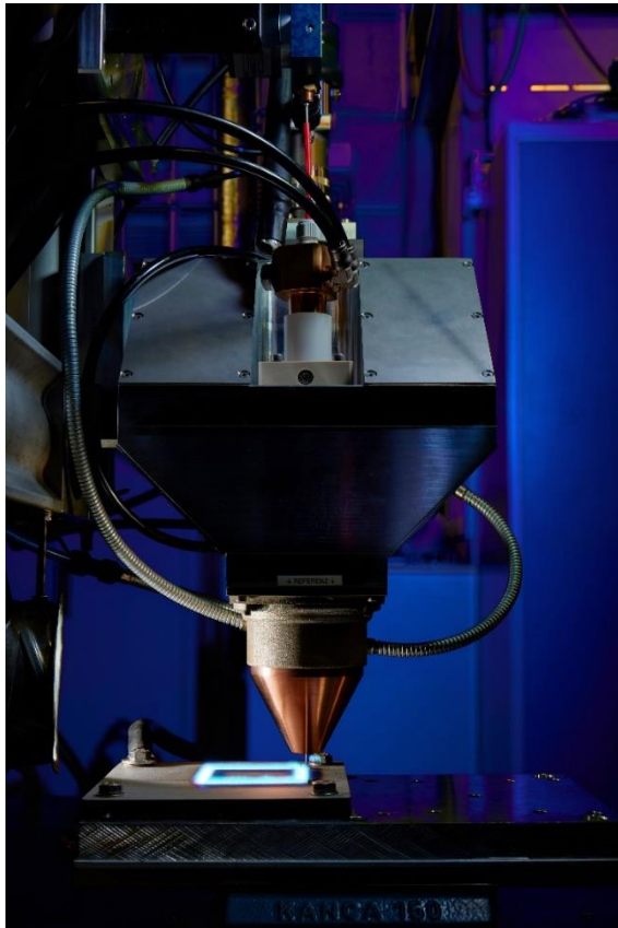
Image 1: The new COLLAR Hybrid Additive Manufacturing process relies on a combination of arc and laser deposition. © Fraunhofer ILT, Aachen, Germany / Volker Lannert.
